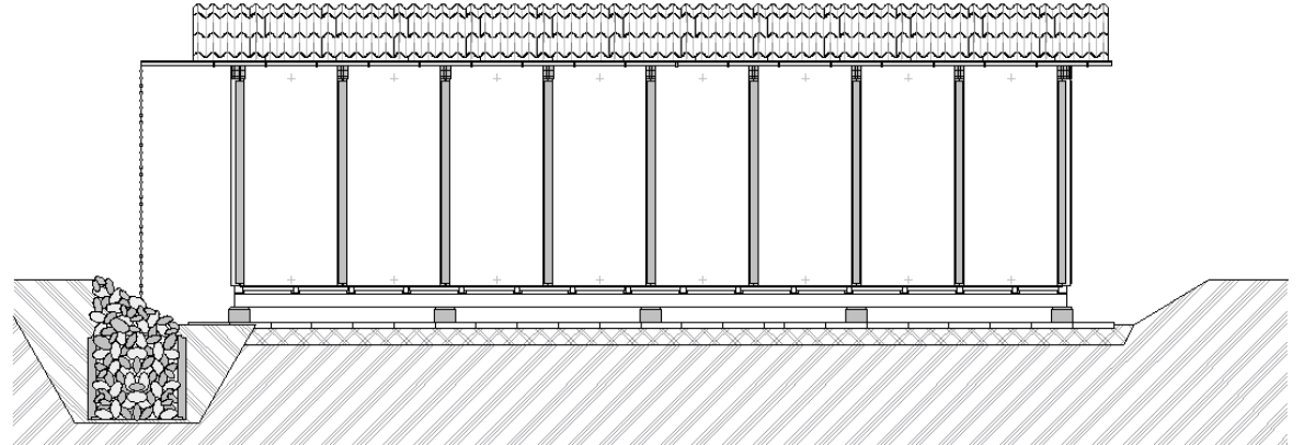
Fassade Nord-West
